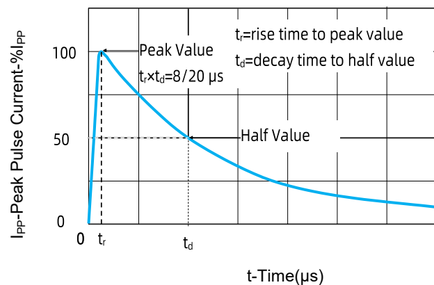
FIGURE 2 Pulse Waveform
