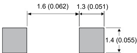
SOD-123FL
