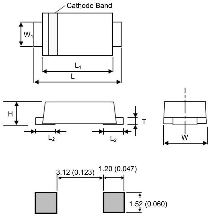
Mounting Pad Layout
