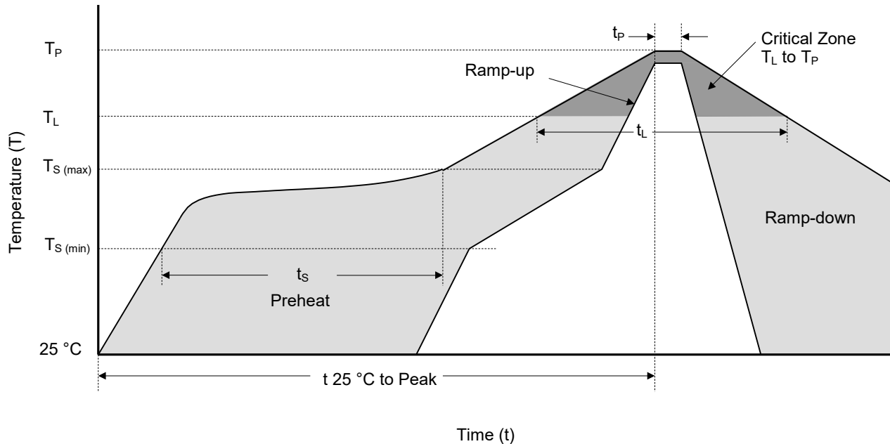
Reflowing Condition
