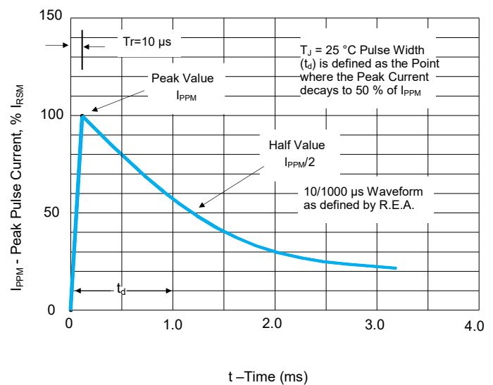
FIGURE 4 Pulse Waveform
