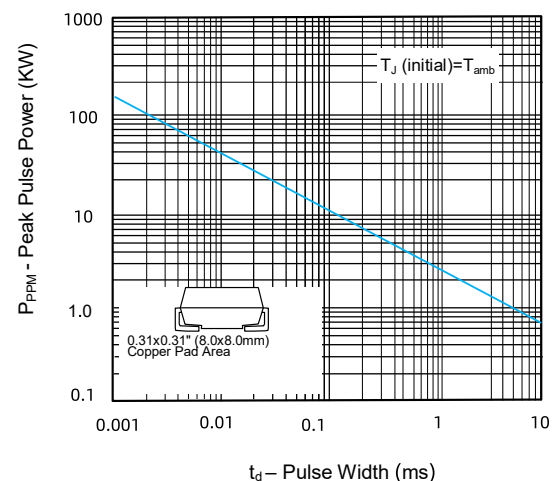
FIGURE 2 Peak Pulse Power Rating Curve
