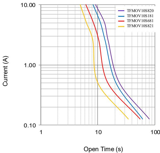
Limited Current Test Curve (UL 1449 4th clause 44.4)
