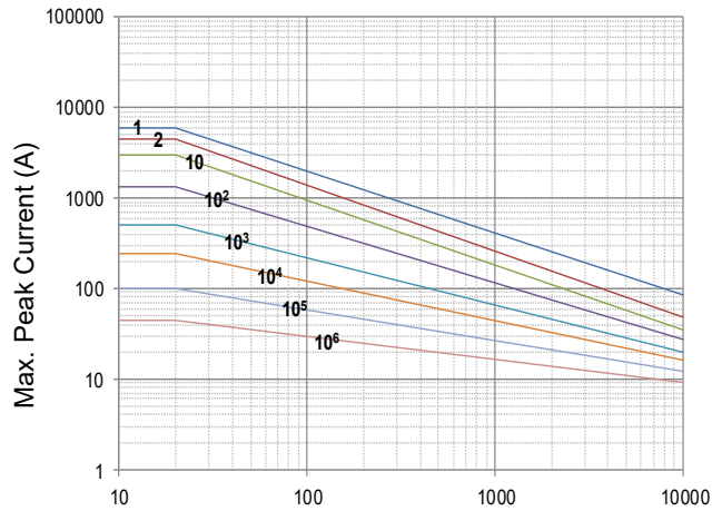
Impulse Duration (μs) SFV25D470KM to SFV25D680KM
