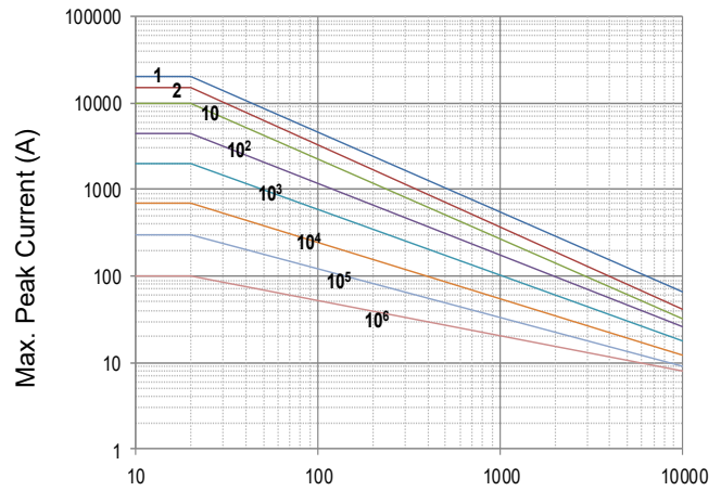
Impulse Duration (μs) SFV25D820K to SFV25D122K
