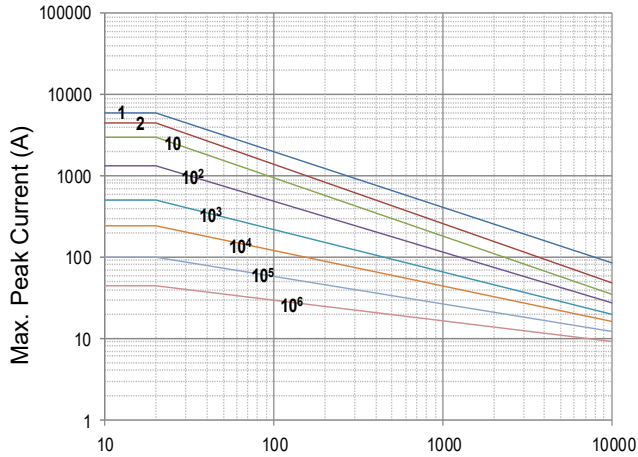
Impulse Duration (μs) SFV25D220K to SFV25D680K
