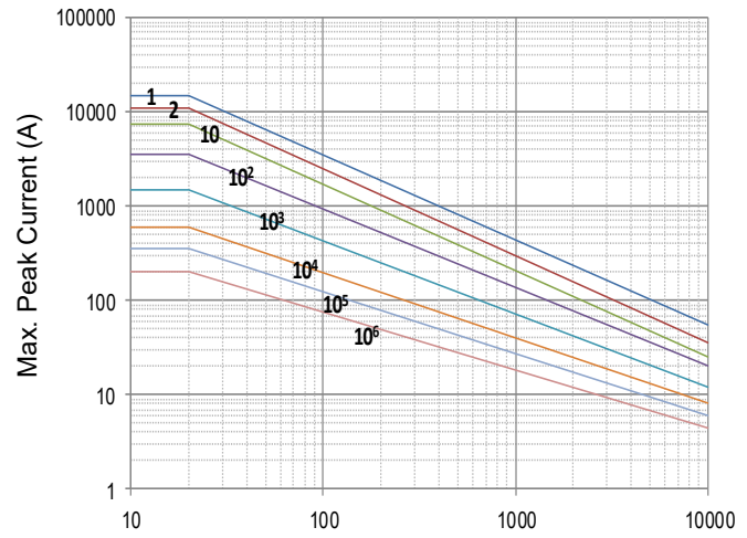
Impulse Duration (μs) SFV20S820K to SFV20S122K
