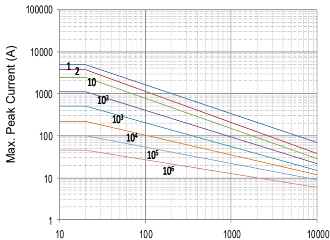
Impulse Duration (μs) SFV20S220K to SFV20S680K
