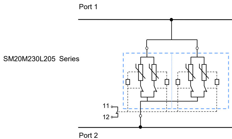
Figure 2 Single protection mode (40 kA)
