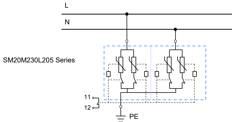
Figure 1 Single-phase circuit common mode protection (20 kA)
