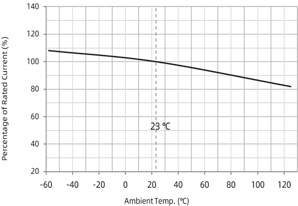
Rated Current Derating Curve (For Reference Only)
