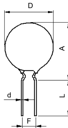
Inward Crimp Lead
