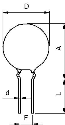
Outward Crimp Lead
