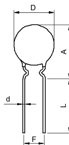
Inward Crimp Lead
